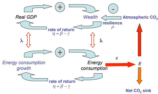
Fig. 4. Schematic illustrating the CThERM framework for economic growth (Garrett, 2011), coupled to atmospheric CO 2 concentrations. Global rates of primary energy consumption rates a are tied to accumulated inflation-adjusted global economic wealth C = \int_0^t P dt' through a constant coefficient \lambda = 9.7 milliwatts per 1990 dollar. Because \lambda is a constant, growth in energy consumption rates da/dt are represented economically by the real, inflation-adjusted global GDP P . Thus, da/dt = \lambda P determines the “rate of return” \eta = d \ln \eta / dt adding to a = \lambda C . E represents the anthropogenic rate of CO 2 emissions, \beta is the source for a positive rate of return \eta due to increasing availability of energy reservoirs. \gamma is the sink for civilization growth driven by environmental degradation. Emissions E determine CO 2 concentrations, subject to land and ocean sinks. CO 2 concentrations act as a negative feedback on economic growth.
