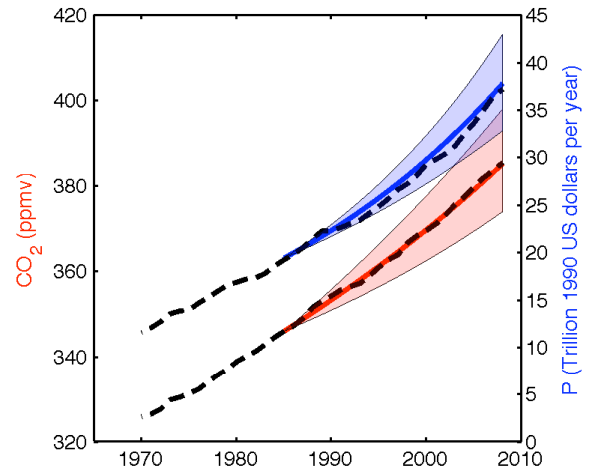
Fig. 5. Based on the CThERM model given by Eqs. (27) to (29), hindcast trajectories and associated uncertainty estimates for the period 1985 to 2008 in a space of atmospheric CO 2 concentrations (red) and global economic production (blue). Observed statistics for the period 1970 to 2008 are shown by black dashed lines. The model is initialized with observed conditions in 1985, and a linear trend in the nominal production coefficient \beta between 1970 and 1984.
