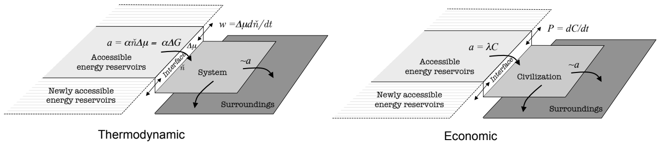
Fig. 1. Schematic for the thermodynamic evolution of an open system, and its hypothesized economic representation. Energy reservoirs, civilization, and its surroundings lie along distinct constant potential surfaces. The number of material units \tilde{n} defining an interface between civilization and energy reservoirs determines the speed of downhill energetic flow at rate a , in proportion to a fixed specific potential difference \Delta\mu and rate coefficient \alpha . The interface itself grows or shrinks at rate w due to a net flux convergence into civilization. In a positive feedback, interface growth at rate d\tilde{n}/dt expands energetic flows a by extending civilization's access to previously inaccessible energy reservoirs at rate da/dt . Fiscally, wealth C is proportional to both the interface size \tilde{n} and the rate of primary energy consumption a . The GWP P represents the net expansion of wealth at rate dC/dt due to interface growth. C and a are linked through a constant \lambda . See the text and Garrett (2011) for details.
