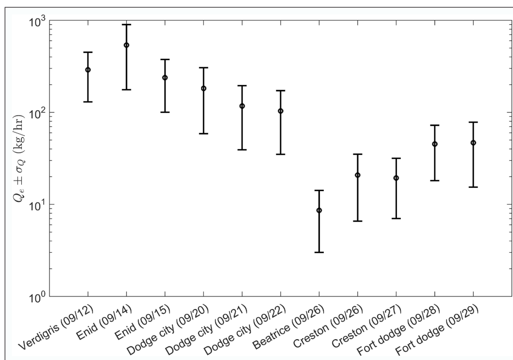
Figure 4: Emission estimates based on daily measurements. Expected methane emission rates and the associated uncertainties ( Q_e \pm \sigma_Q ), in logarithmic scale, derived from the Bayesian approach using daily data collected at each plant. DOI: https://doi.org/10.1525/elementa.358.f4
