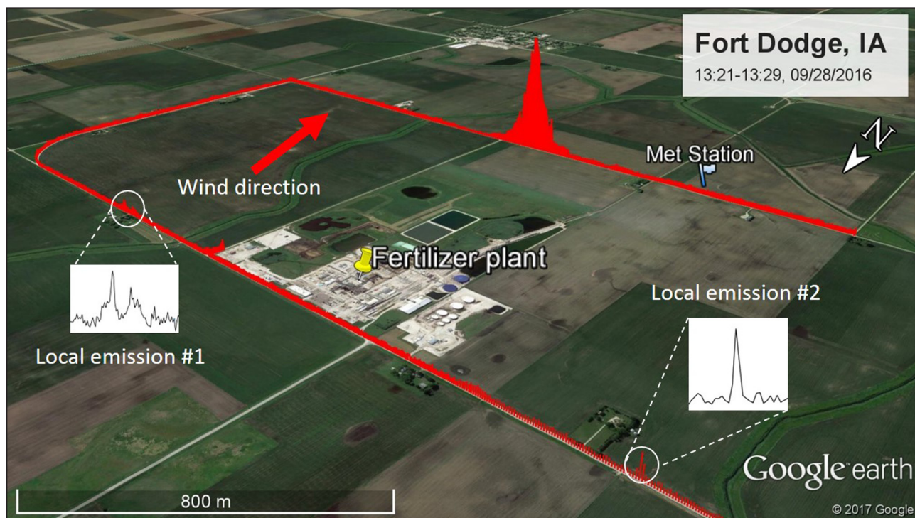
Figure 2: An example of downwind methane plume measurement. A Google Earth representation of an example of methane mixing ratios (red bars) measured by the GSV car along its pass around the ammonia fertilizer plant located in Fort Dodge, IA. Small methane spikes, which may be caused by unground pipeline leaks and not related to emissions from the fertilizer plant, are identified as local emissions. DOI: https://doi.org/10.1525/elementa.358.f2
