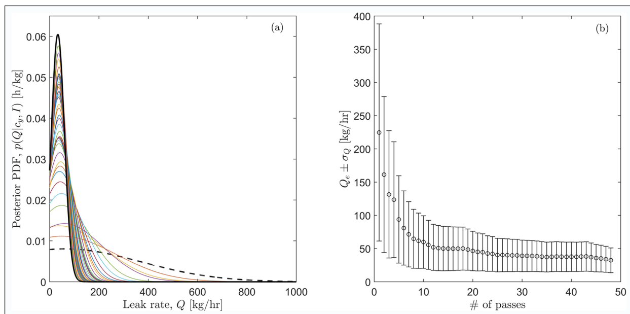
Figure 3: Emission estimates updated after each pass. (a) The posterior PDF, P(Q|c_y, I) , updated after each mobile pass for the plant in Fort Dodge, IA. P(Q|c_y, I) after the first and last pass are highlighted in dash and bold black, respectively. (b) The estimated methane emission rate \pm uncertainty ( Q_e \pm \sigma_Q ) derived from P(Q|c_y, I) after each mobile pass. DOI: https://doi.org/10.1525/elementa.358.f3
