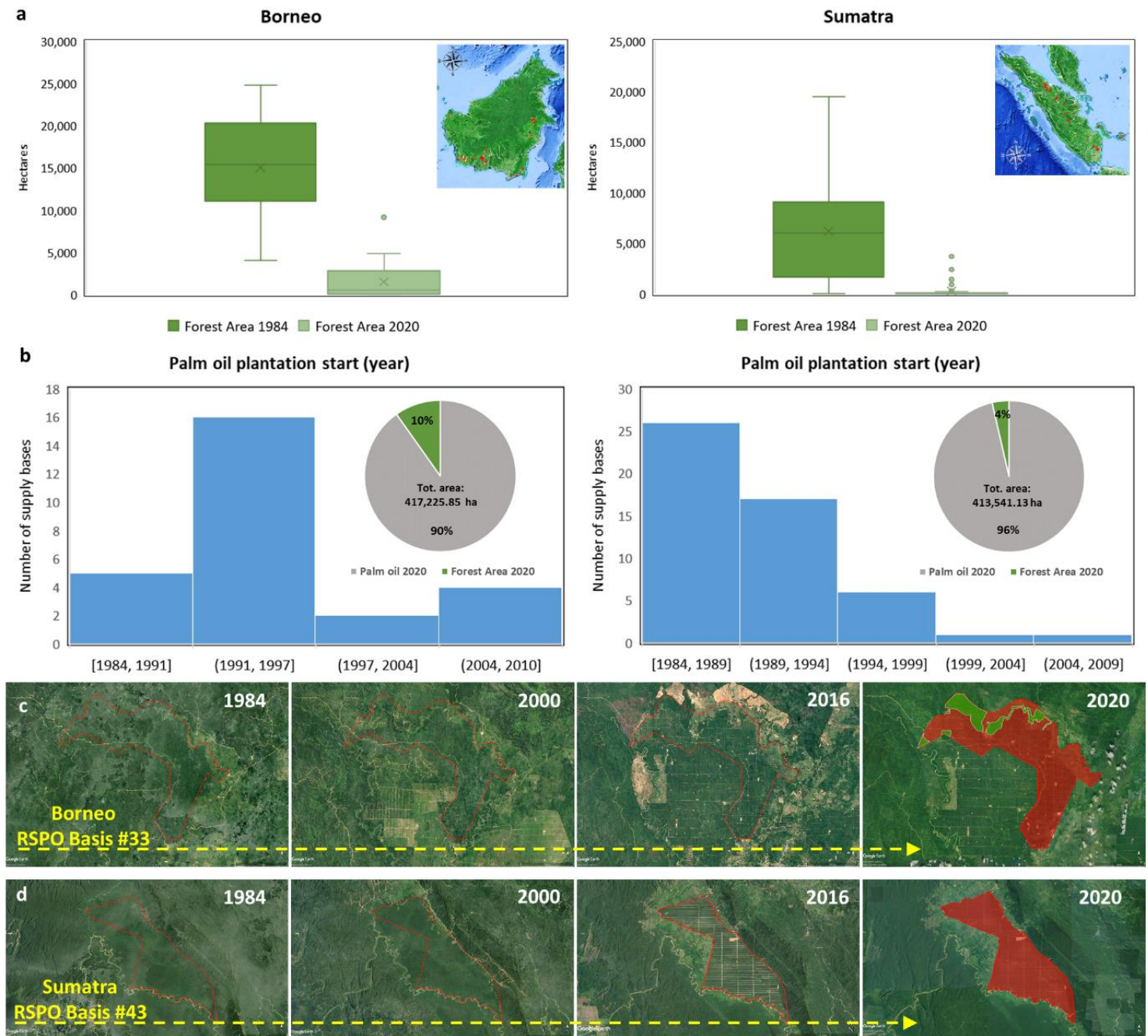
Figure 2 A time-series analysis of satellite images reveals the pattern from deforestation to certification. a) a comparison between 1984 and 2020 forest areas in Bornean and Sumatran RSPO-certified supply bases (red areas in the upper-right panel; boxplots shows the distribution of forest areas between upper and lower quartiles, the mean as an X and outliers as points outside the “whiskers”, which indicate the variability); b) the average period when oil palm plantation started (year) in certified bases and the percentage of the area currently occupied by oil palm and forests in 2020 (in the smaller pie charts) over the total; c) time series of high-resolution satellite images from 1984 to 2020 of two sample bases (see Supplementary Figures 2 and 3
